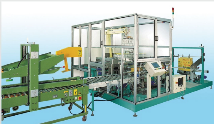
Flexible Pick & Place with Sealing System
